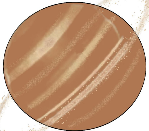
Saturn
